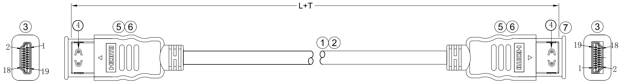
A FRONT VIEW
